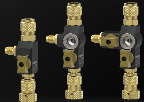
Valve Core Removal Tools VC1, VC1G, VC2G
