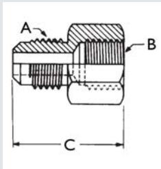
Half Union - Flare to NPTFI
